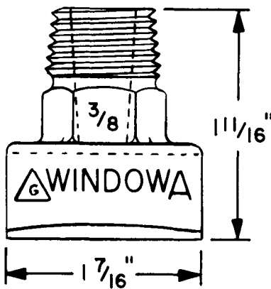
WINDOW SPRINKLER, ISSUE A.
