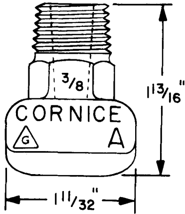
CORNICE SPRINKLER, ISSUE A.
