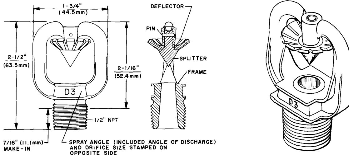
FIGURE A TYPE D3 PROTECTOSPRAY NOZZLES
